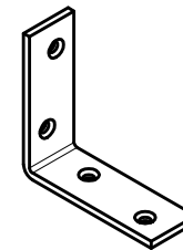
ST1= 40x40x2 (4x)
